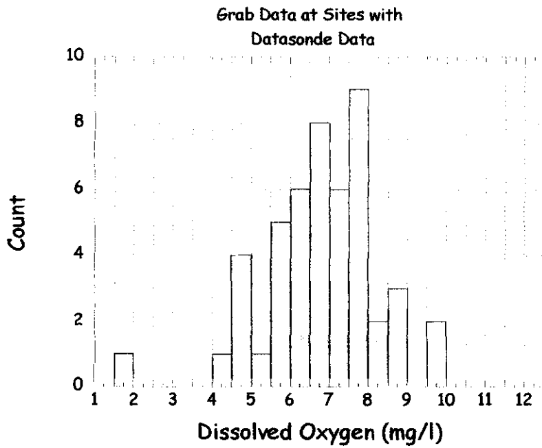
Figure 9. Histograms of minimum dissolved oxygen data (mg/l) at stations with IBI values of 40-49 (WWH range) from a statewide Ohio data set (top) and a subset of sites that also had datasonde data (bottom).
